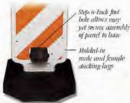
24" x 8" TrafFix Vertical Panel Barricade with light and 43lb. recycled rubber base 34000 Series
