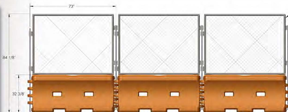
45032-WWF Fence Panel for TrafFix Water-Wall
