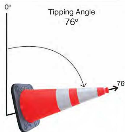
7 lb. Enviro-Cone
